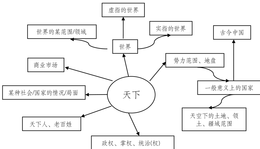
图4 “天下”义项语义网络
